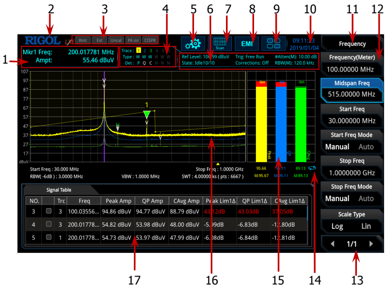
Figure 5 User Interface (EMI Mode)
