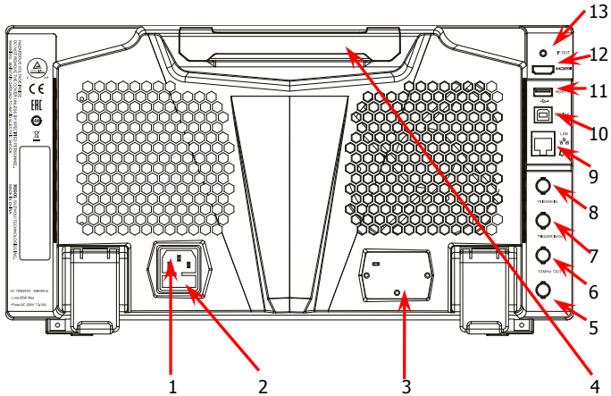
Figure 2 Rear Panel
