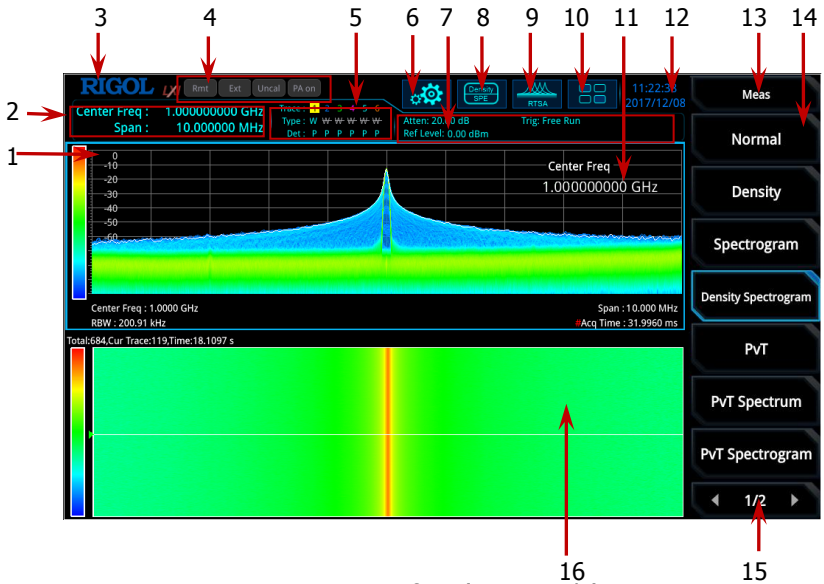
Figure 4 User Interface (RTSA Mode)
