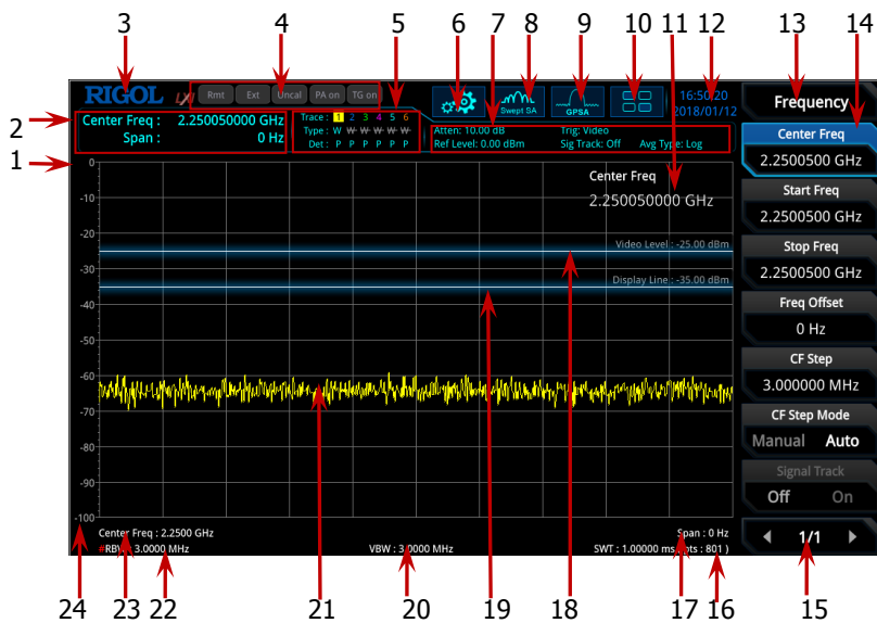
Figure 3 User Interface (GPSA Mode)
