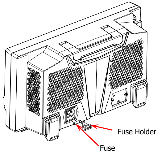
Figure 10 Fuse Replacement
