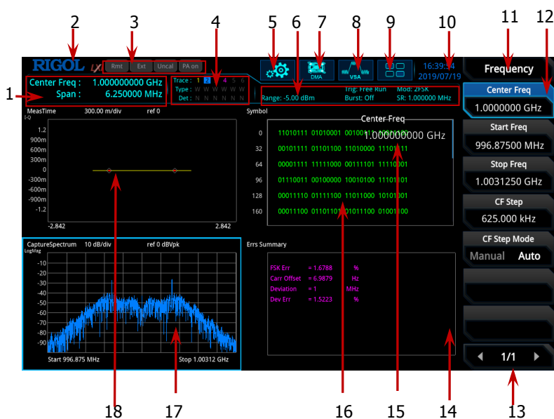
Figure 6 User Interface (VSA Mode)
